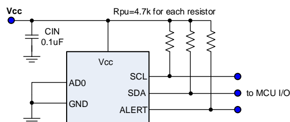
Figure 15. Sensor typical application
