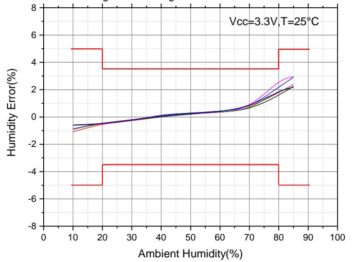
Figure 10. Humidity Error vs Ambient Humidity
