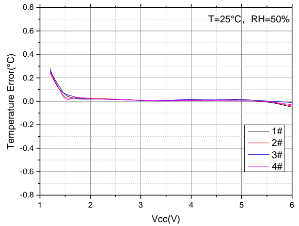
Figure 12. Temperature Error vs. Vcc(RH=50%)
