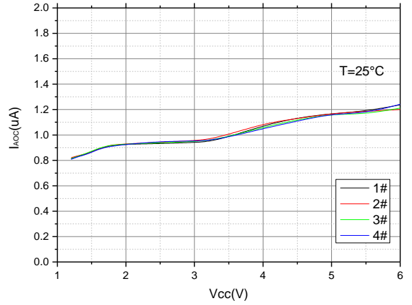
Figure 8. Average Current vs Vcc
