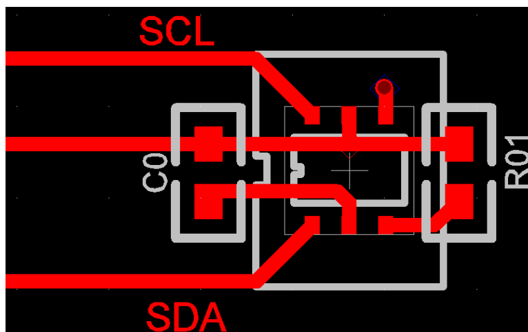
Figure 17. Sensor PCB layout example
